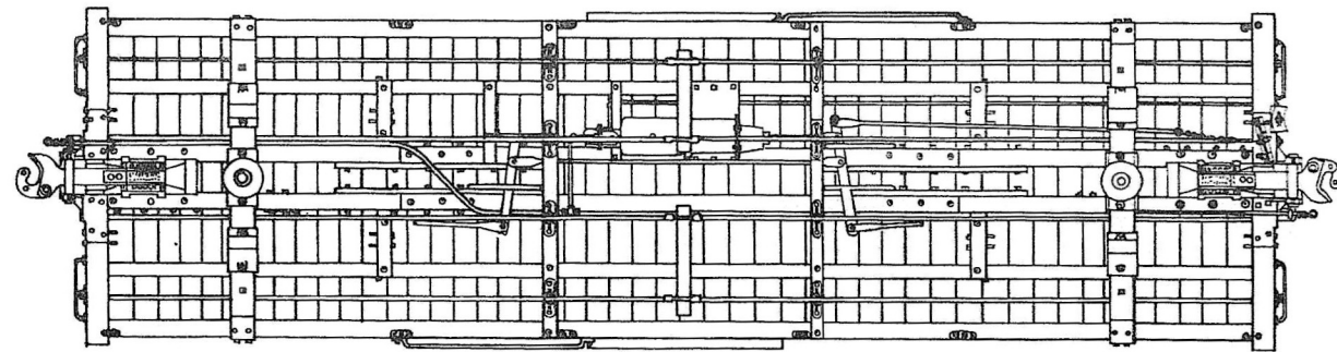
UNDERFRAME VIEW 1A
