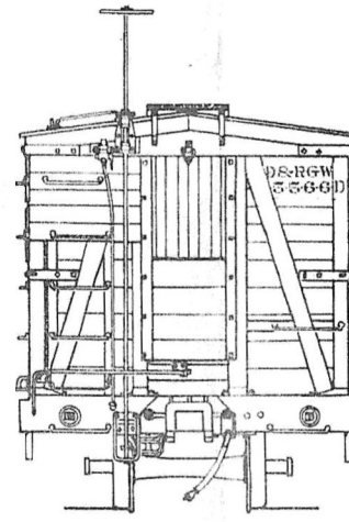
"A" END VIEW
