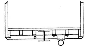
Section Thru Brake Cylinder And Mount
